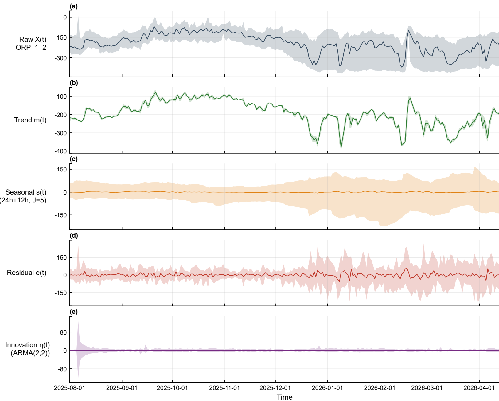
Full-span daily overview — ORP_1_2 (pre_anoxic_front, min) [2025-08-01~2026-04-13]
